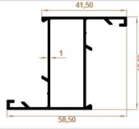
Aldoks (Dar) Kanat Profili Aldox (Narrow) Airfoil
