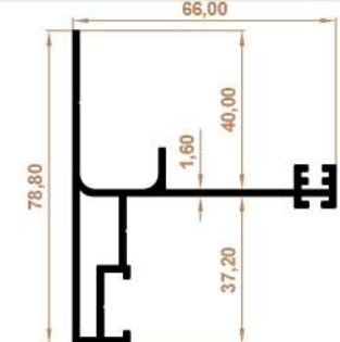
Yan Ray "T" Profil Side Rail "T" Profile
