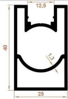
40x25 Tek Kanallı 40x25 Single Slot
