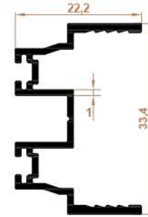
Düz Kapak Mentеше Profil Flat Cover with Hinge Profile
