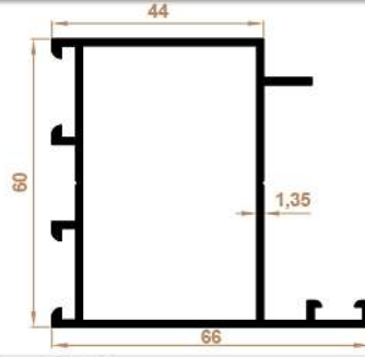
C60 Kanat Profili C60 Airfoil
