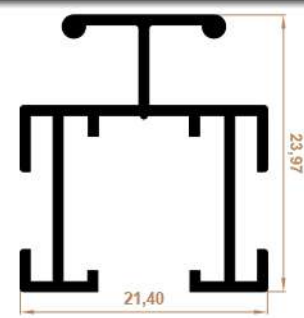
Çiftli Orta Profil Double Middle Profile
